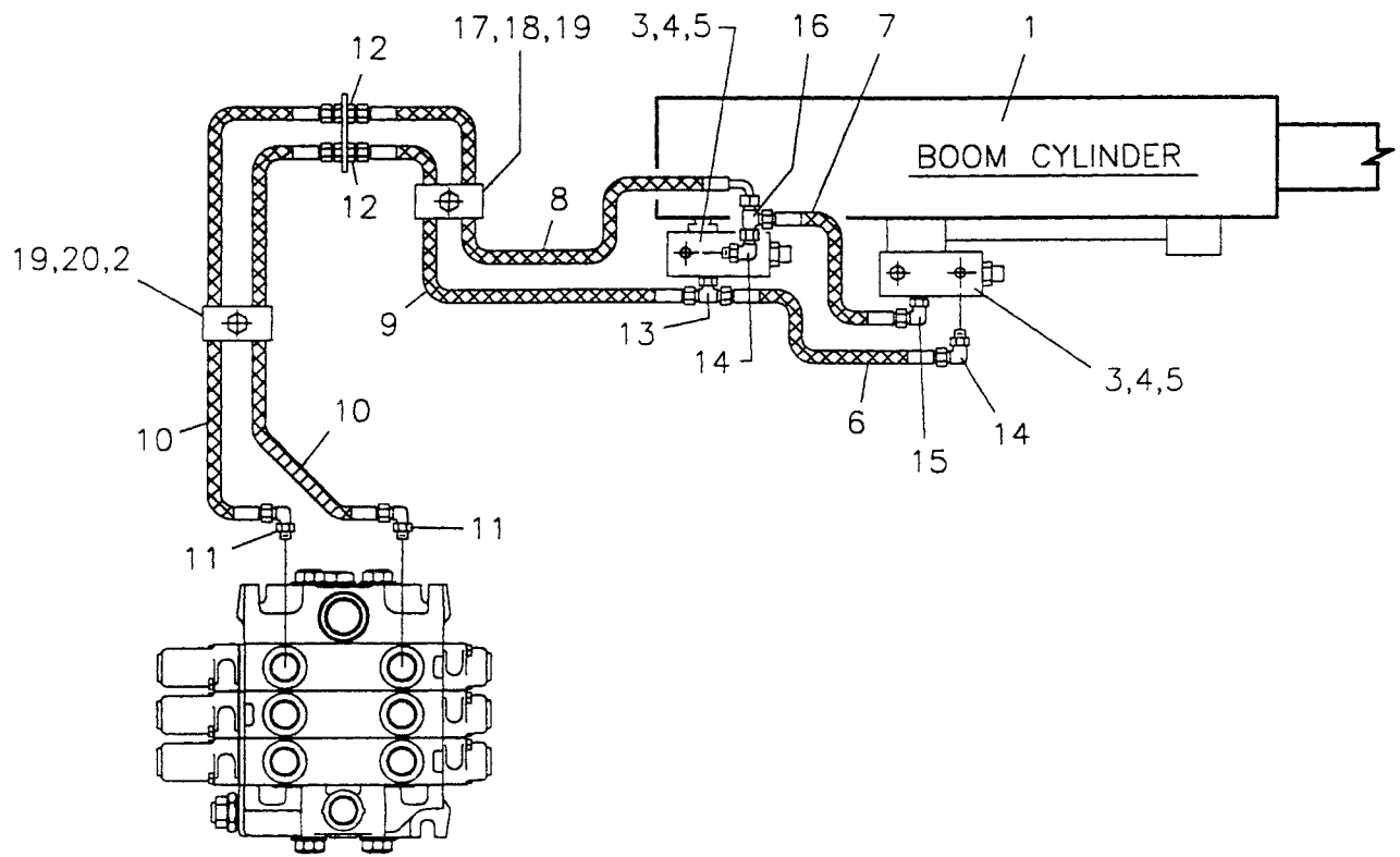
MAIN VALVE ASSEMBLY
